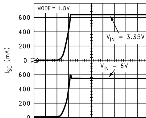
TIME (500 μs/DIV)
